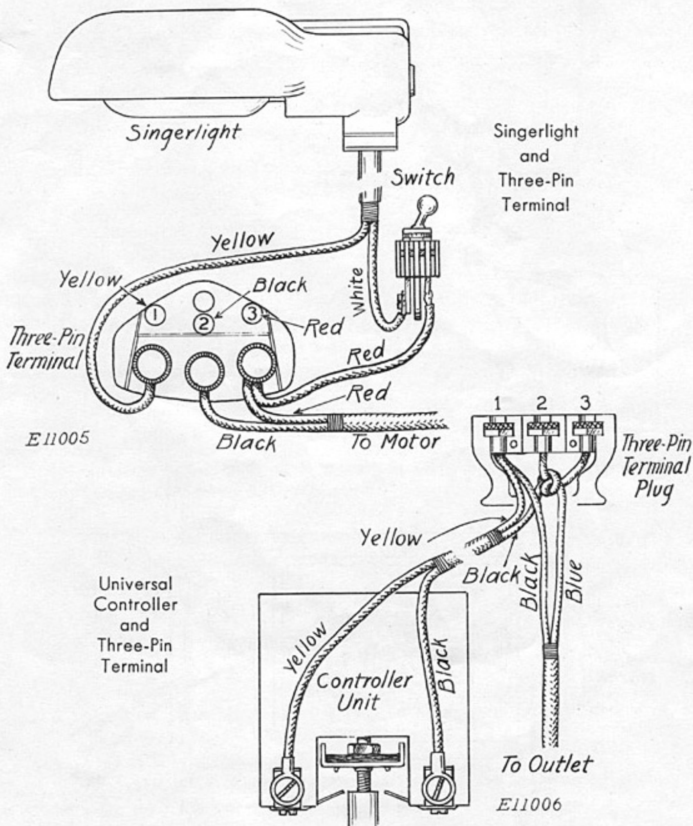
Wiring Diagrams of Connections to Series 3 and Series CA6 Motors, used with Singer 221-1 Machine.
