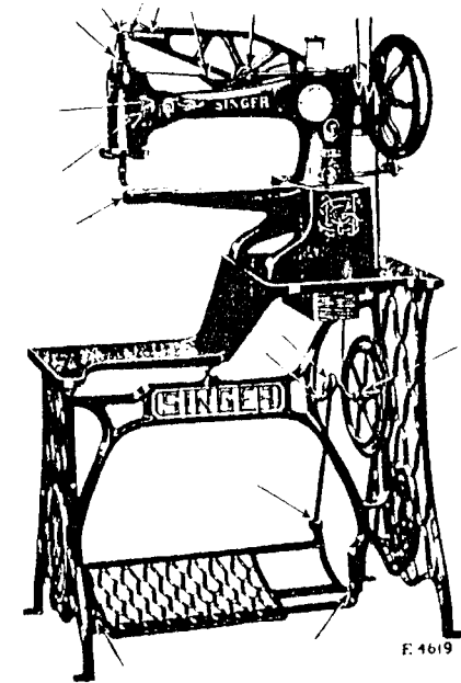
FIG. 10. OILING PLACES IN MACHINE AND STAND
